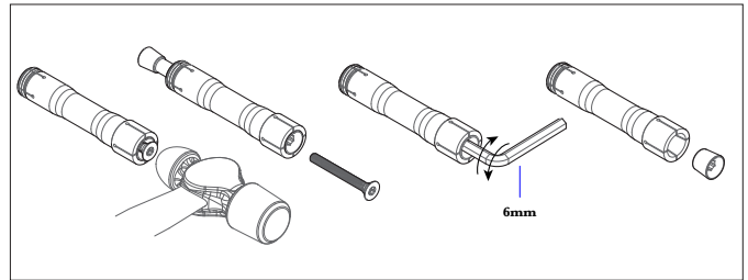
Wedge Removal: (shown removed from link for clarity)
