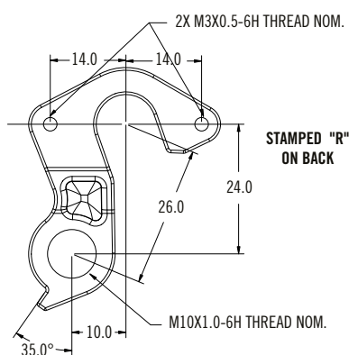
KP255/ - KIT, DER. HANGER, SINGLE SIDED RD2
