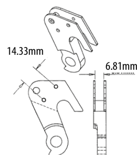
A239X/EBO - KIT, DER. HANGER, MTN.
