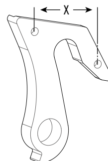
KP093/ - KIT, DER. HANGER, BAD BOY (X = 30.55 mm)
